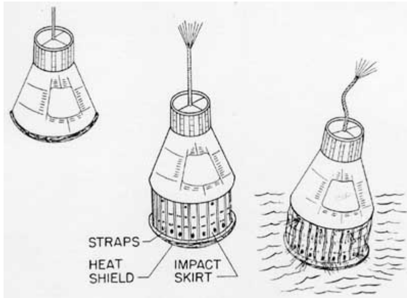
Figure 46. Impact attenuation.
