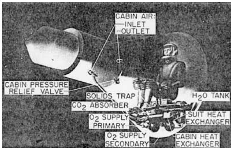
Figure 38. Mercury environmental control system.
