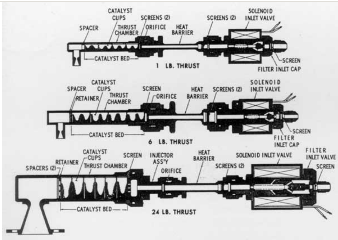
Figure 30. Reaction control thrust chamber.
