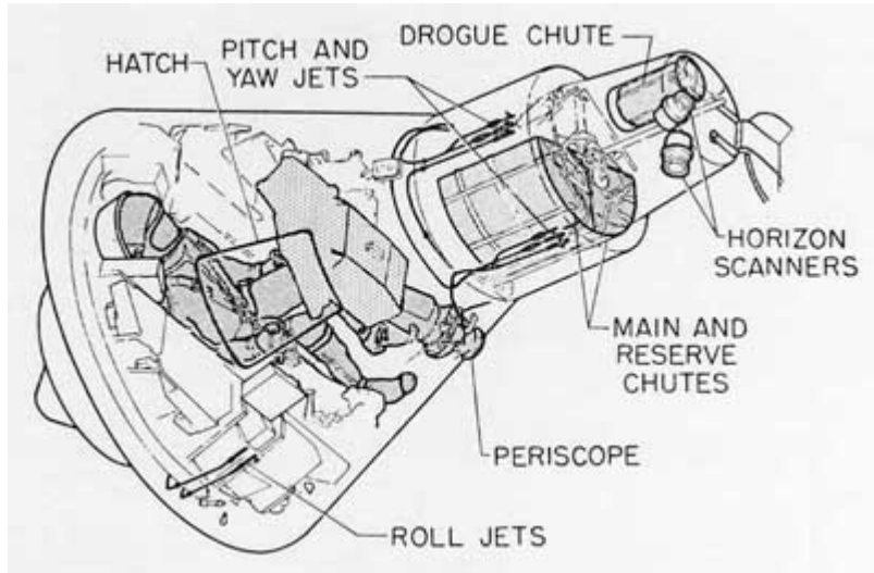
Figure 15. Spacecraft interior arrangement.
